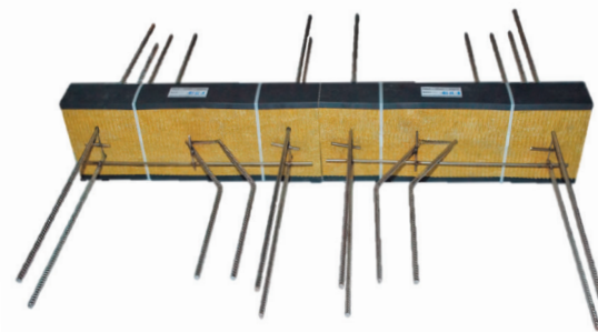
BASYCON Querkraftanschlüsse SeismoLock®
