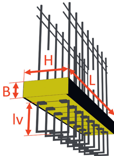
Normalkraftanschlüsse
