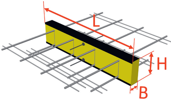
Kragplattenanschlüsse
